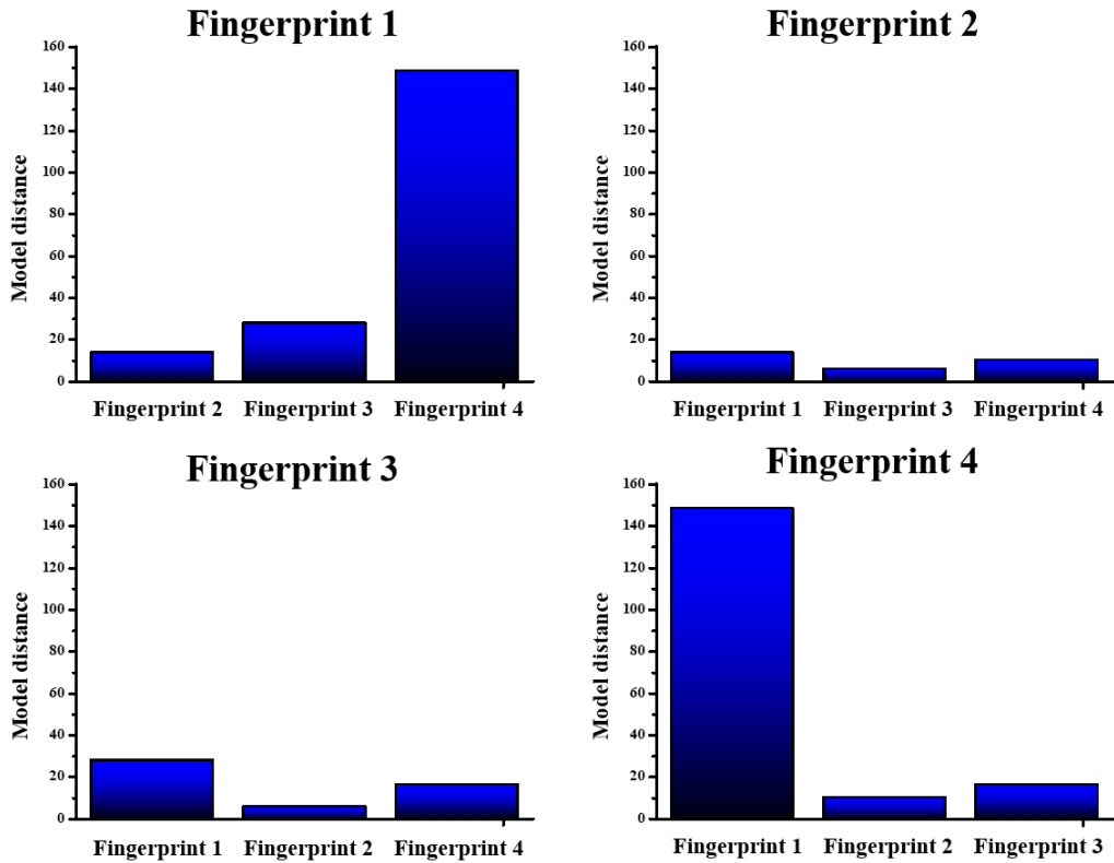
Fig. 4. Model distance using SIMCA method.
