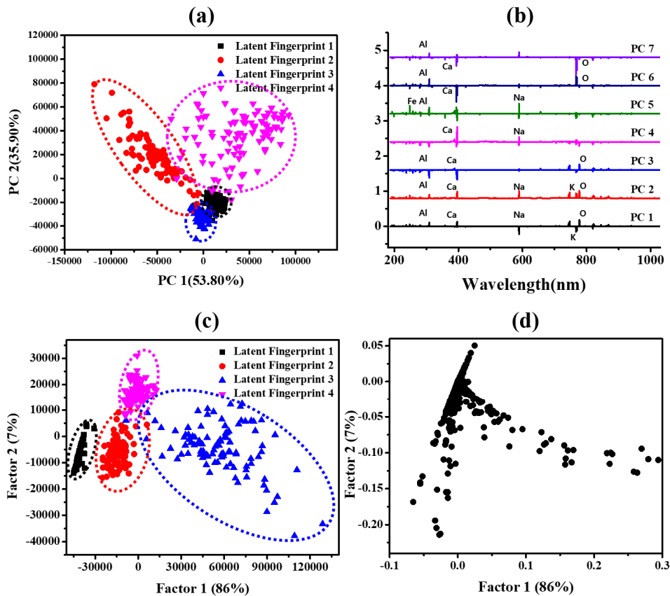
Fig. 3. (a) The results of PCA plot, (b) the results of extracted PCs, (c) the results of PLS method, and (d) the PLS loading plot.
