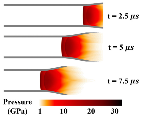
Fig. 9 Pressure contours of 25% aluminized HMX confined rate stick simulation with aluminum particle diameter 7\mu\text{m} .
