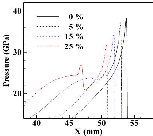
Fig. 7 Detonation velocity decreased by aluminizing with particle diameter 7\mu\text{m} at t = 6\mu\text{s} .
