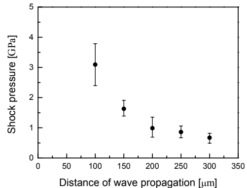
Fig. 10 Shock pressure according to the distance of wave propagation within a stainless steel 304 target.
