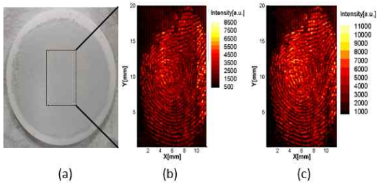
Fig. 11. Pellet soil sample 1(a), chemical mapping about latent fingerprint (766.587 nm)(b), and (770.047 nm)(c)
