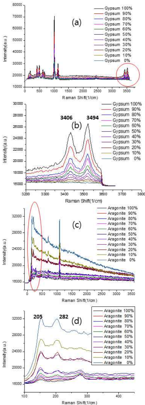
Fig. 6. Raman spectrum about sample 1 (a) and (b), Raman spectrum about sample 2 (c) and (d)
