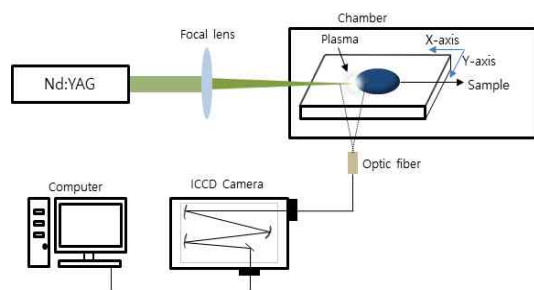
Fig. 1. LIBS Experimental Setup
