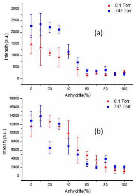
Fig. 8. Hydrogen intensity(656.272 nm) (a), Oxygen intensity(397.325 nm)(b) from LIBS at 0.1 torr about mixture of Gypsum and Anhydrite
