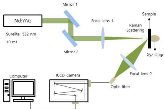
Fig. 2. Raman Experimental Setup
