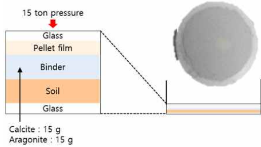
Fig. 3 Making method of soil pellet sample
