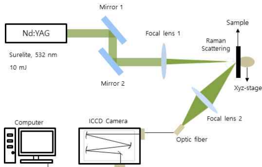
Fig. 2 Raman Experimental Setup
