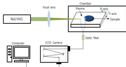
Fig. 1 LIBS Experimental Setup
